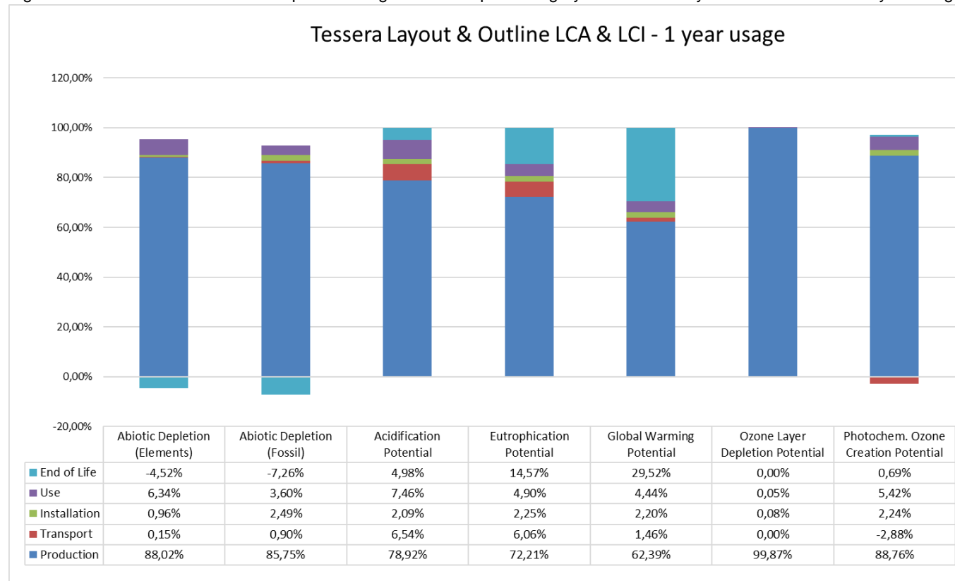
Figure 4: relative contribution of each process stage to each impact category for Tessera Layout & Outline for a one year usage.
